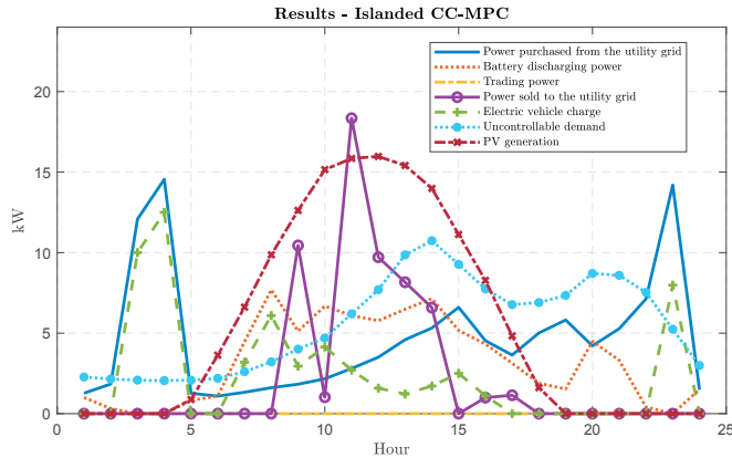
Fig. 2. Results islanded test.
