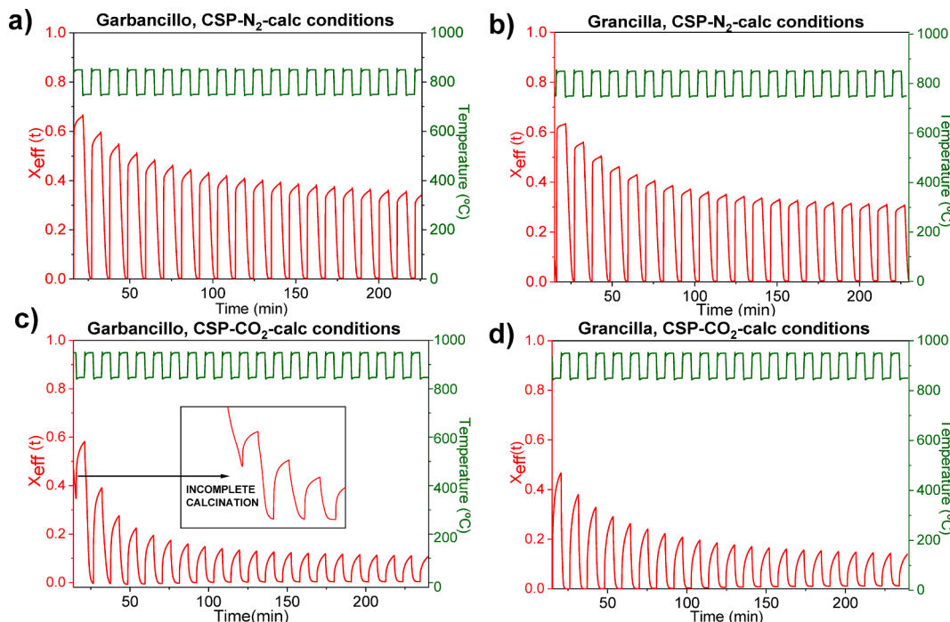
Fig. 6. Time evolution of temperature and effective conversion for multicyle CaL tests conducted under CSP-N 2 -calc conditions and CSP-CO 2 -calc conditions.
